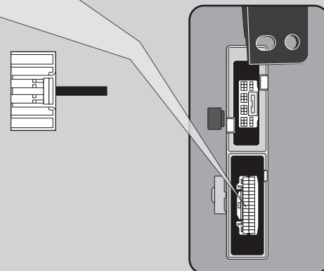
LF Control Module (Passenger Kick Panel) 3
