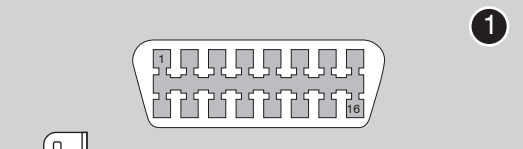
OBD-II Connector
