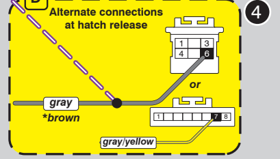
Hatch Release
