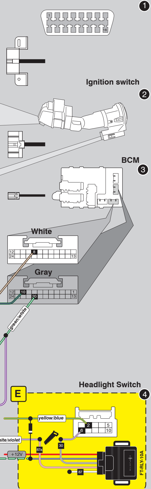
OBD-II Connector 1
