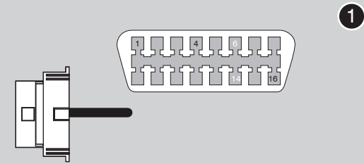
OBD-II Connector 1
