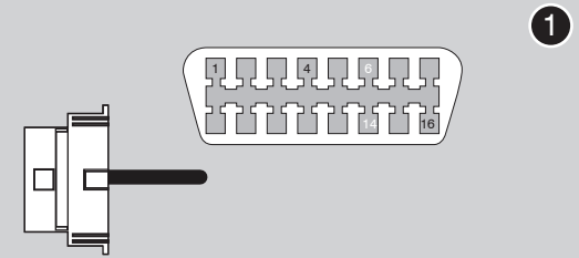
OBD-II Connector
