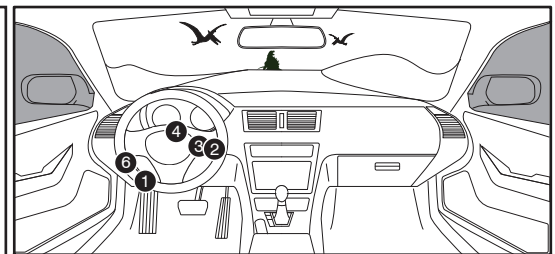
OBD-II Connector
