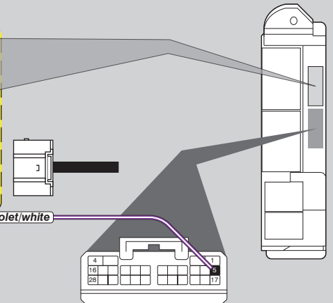
Hybrid ECU RIGHT OF DASH FUSEBOX 3
