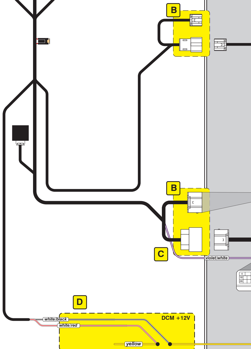
Steering Lock Connector
