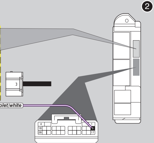
Main Body ECU
