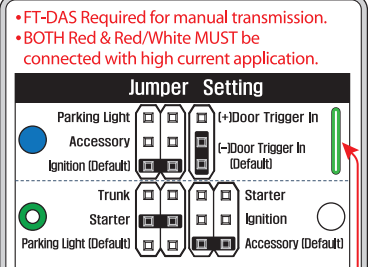
CM7000/7200 Cut loop for A/T
